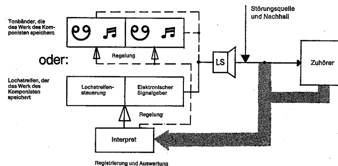
Blockschema:
