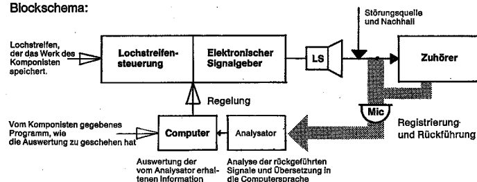
Blockschema:
